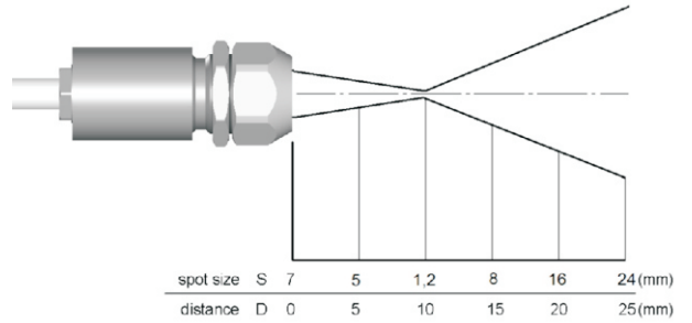
10:1 optics with CF-lens
