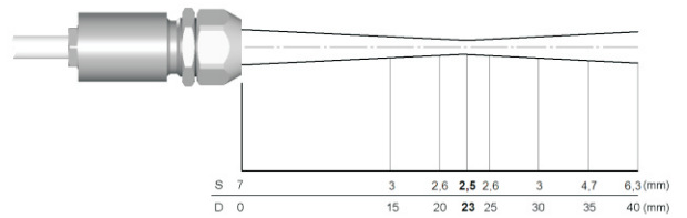
2:1 optics with CF-lens chart
