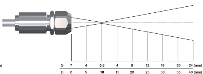
Optics CT LT CF, D:S = 22:1 (far field = 1,5:1)
