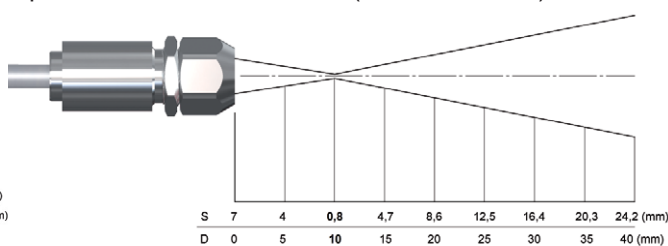
Optics CT LT CF, D:S = 15:1 (far field = 1,5:1)
